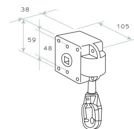
GEARBOX 7:1 (mm)
